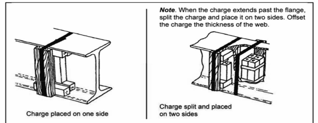
Figure 3-7. Placing Charges on Steel Members
